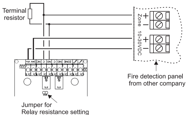
Figure 3. Connection with fire detection panel from other company
