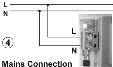
Mains Connection
