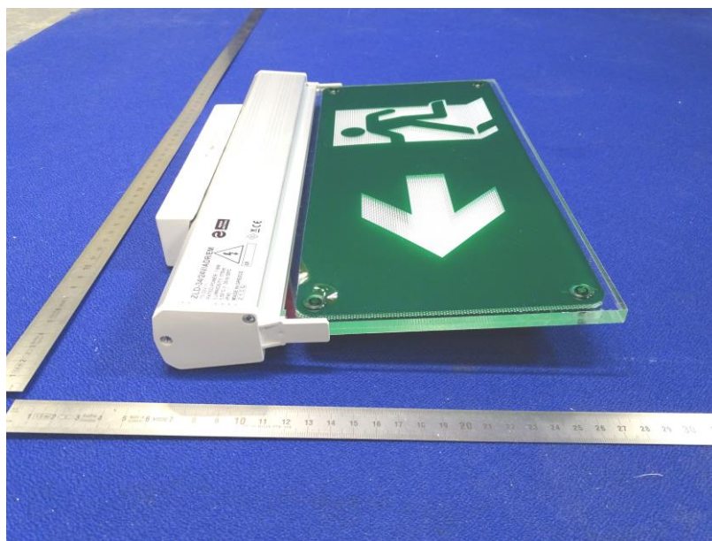
Photograph 4: Luminaire Overview – Emergency Exit Safety Sign Model No. ZLD-34/24V/ADR/EM (Side Profile)
