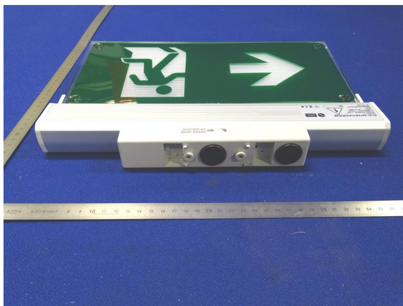
Photograph 3: Luminaire Overview – Emergency Exit Luminaire Model No. ZLD-34/24V/ADR/EM (Side Profile)
