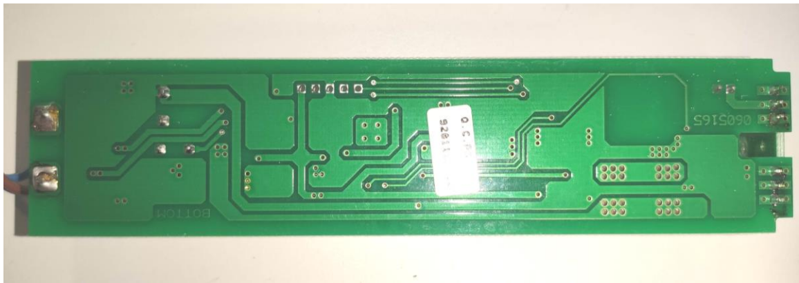
Photograph 6: Built-in lamp controlgear (Bottom)
