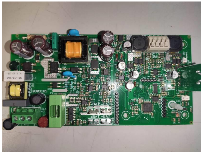
Photograph 7: Integrated lamp control gear (Top)
