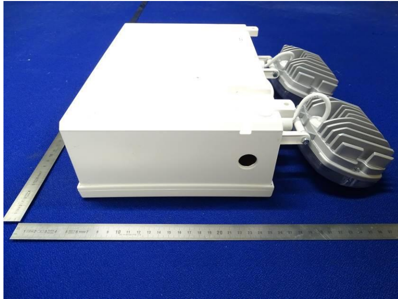
Photograph 5: Luminaire Overview – Two spot emergency luminaire Model No. GRL-37/180/WP/ADR (Side Profile)
