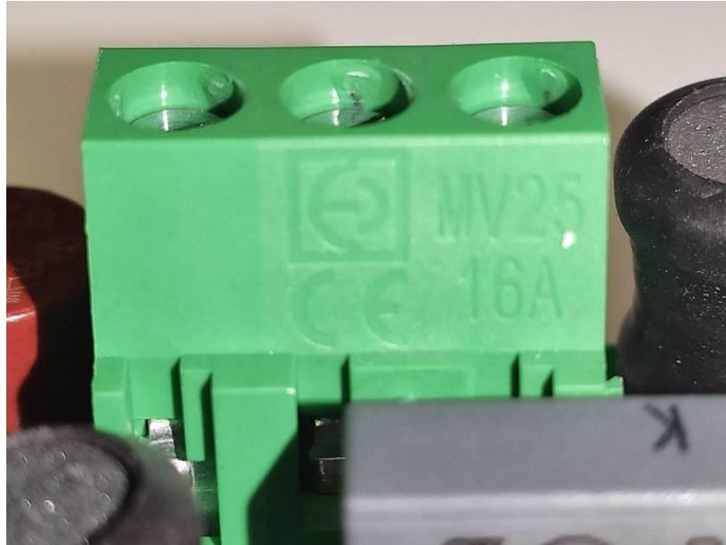
Photograph 13: Mains input terminal
