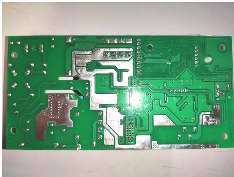
Photograph 8: Integrated lamp control gear (Bottom)
